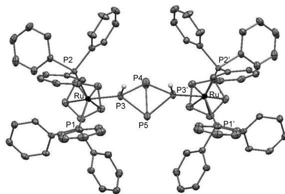
Figure 3. Geometry of the dimetallic cationic complex in 3 in the crystal structure of the solid solution of [\{\text{CpRu}(\text{PPh}_3)_2(\mu^{1,3},\eta^{1:1}\text{-P}_4\text{H}_2)\}(\text{OTf})_2] ( 3 ) and [\{\text{CpRu}(\text{PPh}_3)_2(\mu^{1,3},\eta^{1:1}\text{-P}_3\text{H}_5)\}(\text{OTf})_2] ( 4 ) in a molar ratio of 1:2 with 30% probability thermal ellipsoids. Primed atoms are related to the corresponding unprimed ones by a mirror plane. Hydrogen atoms of phenyl groups and Cp ligands are omitted for clarity. Selected bond lengths [Å]: Ru–P1 2.3404(8), Ru–P2 2.3411(8), Ru–P3 2.2731(8), P3–P4 2.163(2), P3–P5 2.121(3), P4–P5 2.312(6), P3...P3' 3.322(1).
